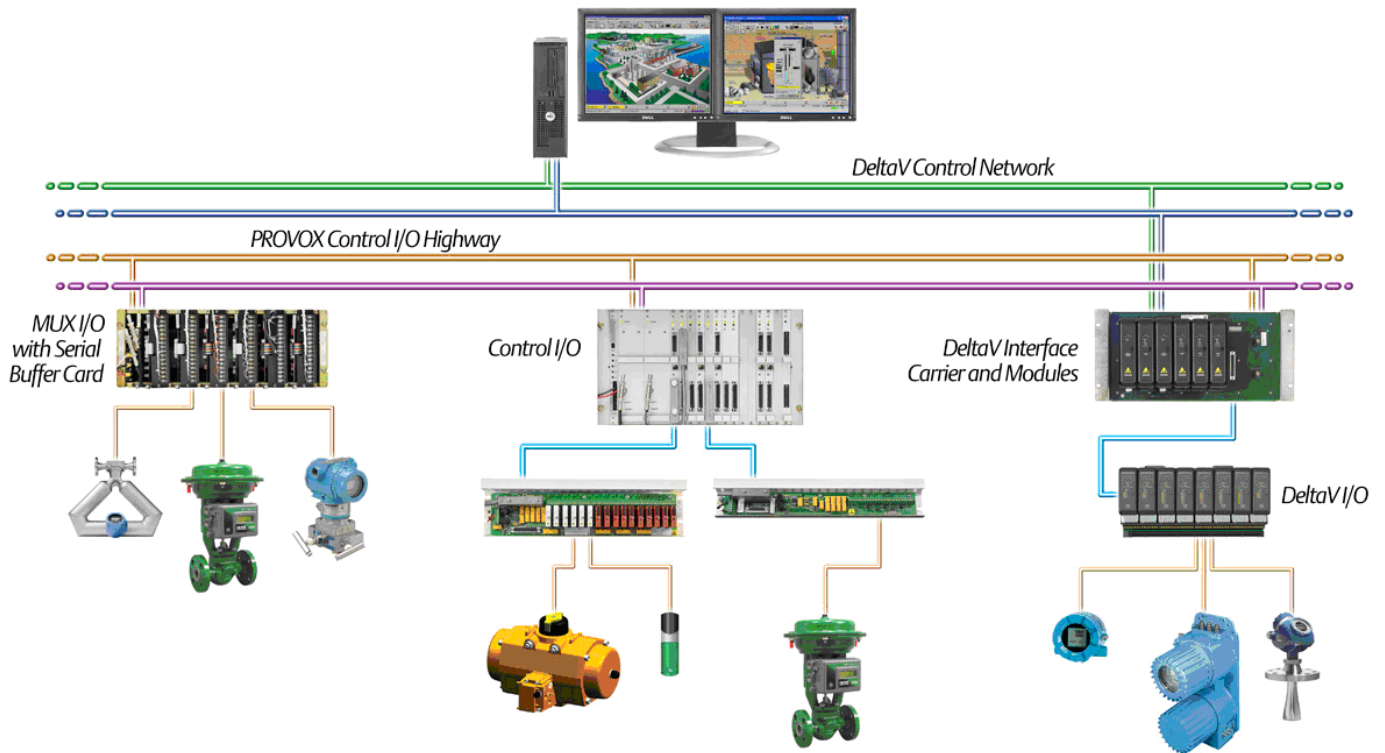
DeltaV Controller Interface for PROVOX I/O
