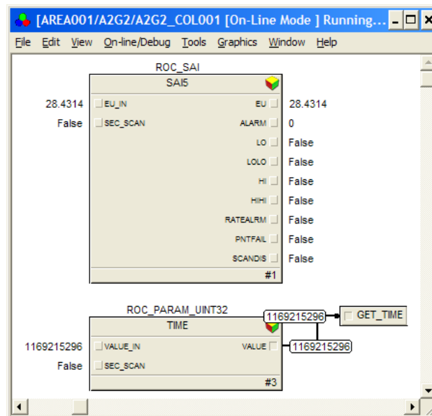
ROC analog input function block.
