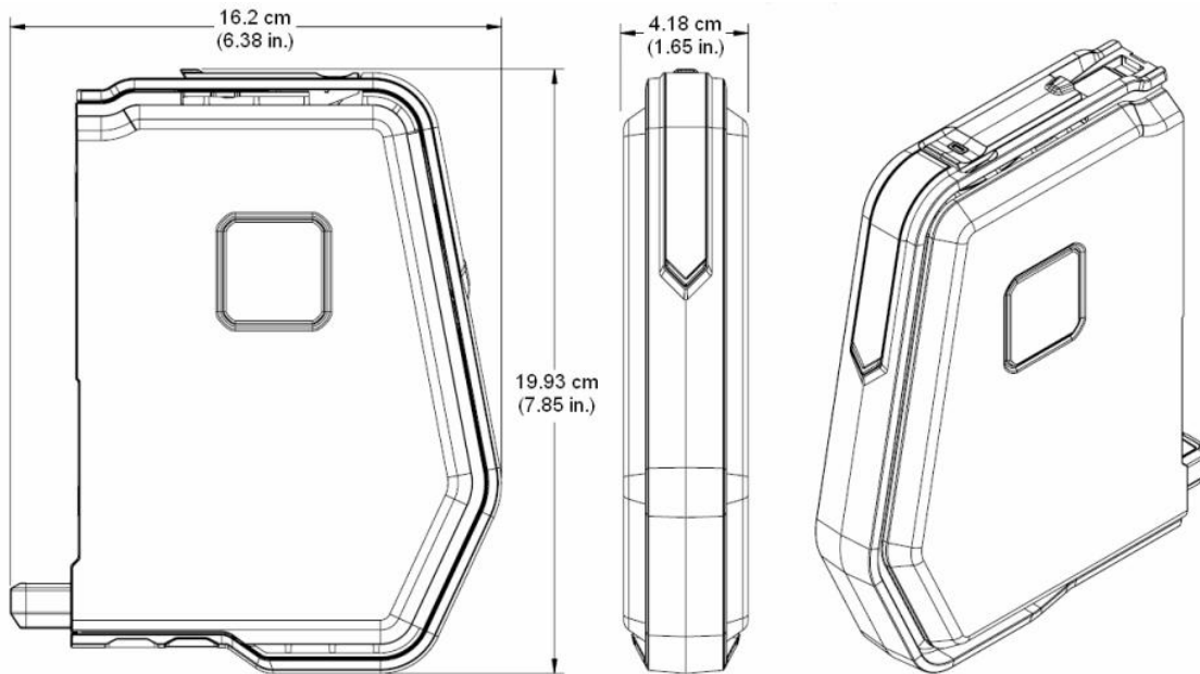
S-series controller hardware dimensions
