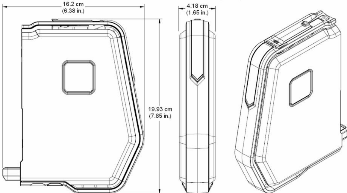
S-series controller hardware dimensions
