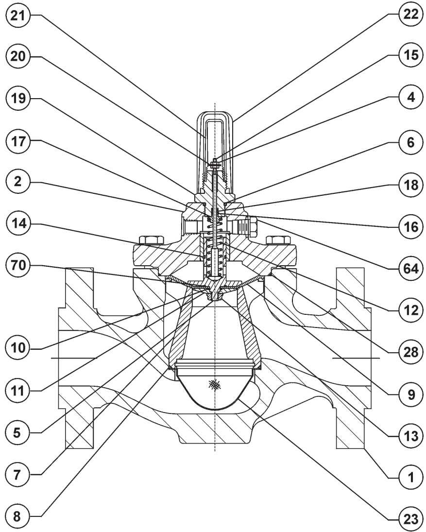
MAIN VALVE ASSEMBLY
